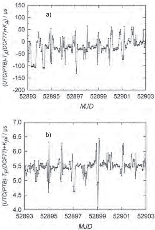
Figure 11: The time differences UTC(PTB) - T_A(DCF77) + K_A ;
