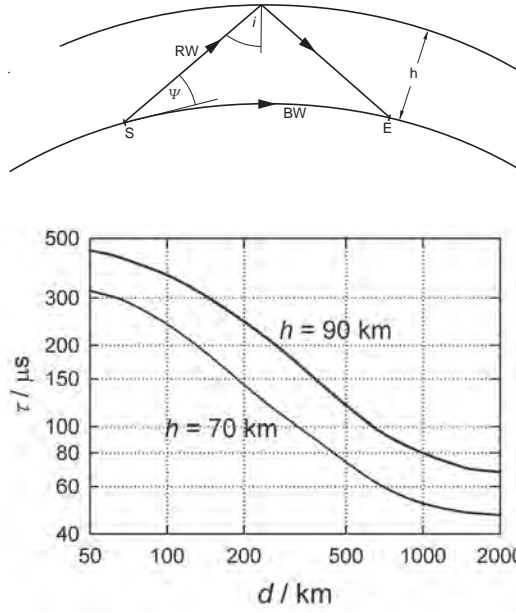
Figure 12: Schematic view of the propagation of the ground wave and the sky wave between the transmitter and the receiver; h : height of the ionospheric D layer, \psi : elevation angle, i : angle of incidence onto the D layer.
